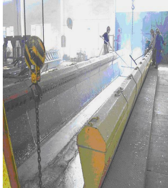
13M in Length, Galvanizing Kettle
